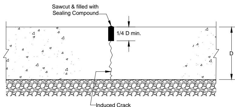
Figure 4. Contraction joint cut into a concrete alley and filled with a flexible liquid sealer.
