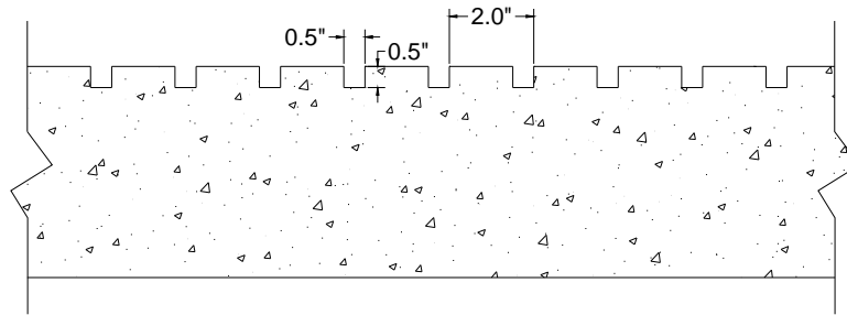
Figure 2. Cross sectional view of a parallel grooved concrete floor with recommended dimensions.
