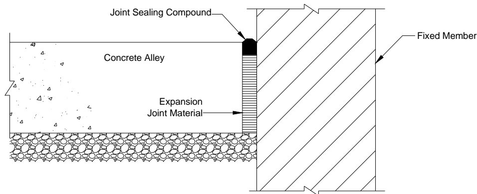
Figure 3. Expansion joint located between a barn alley and a fixed part of the barn such as a structural column.
